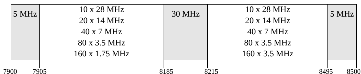
Figura 13. Brezi i frekuencave 7900 – 8500 MHz
