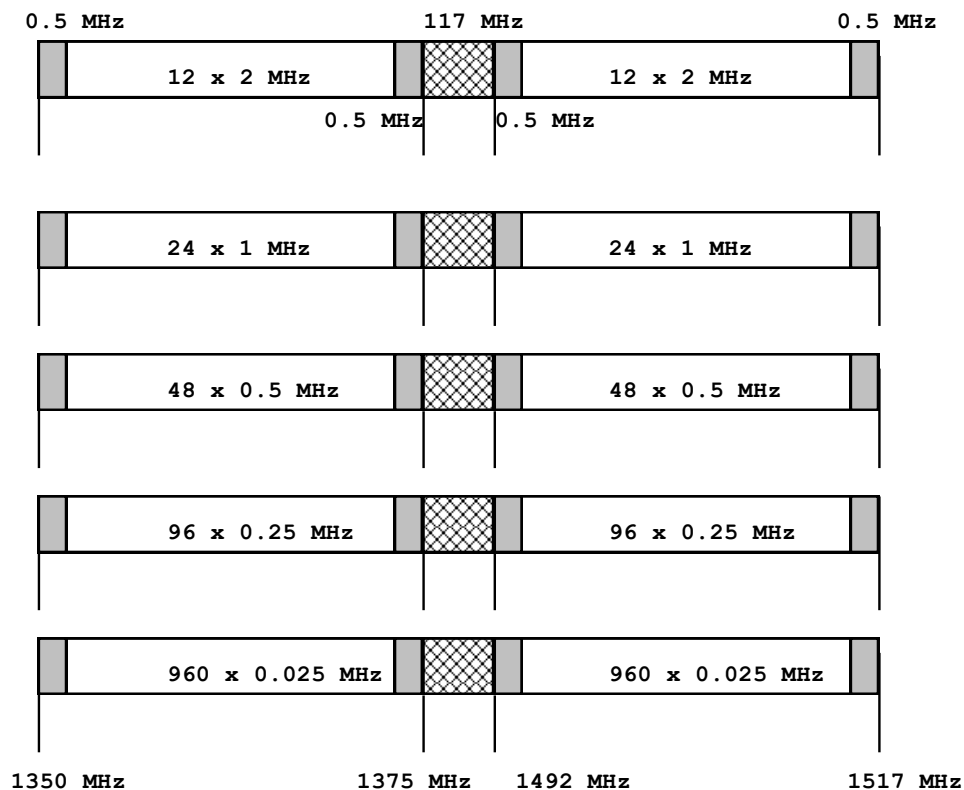
Figura 2. Brezi i frekuencave 1350 – 1375 MHz / 1492 – 1517 MHz
