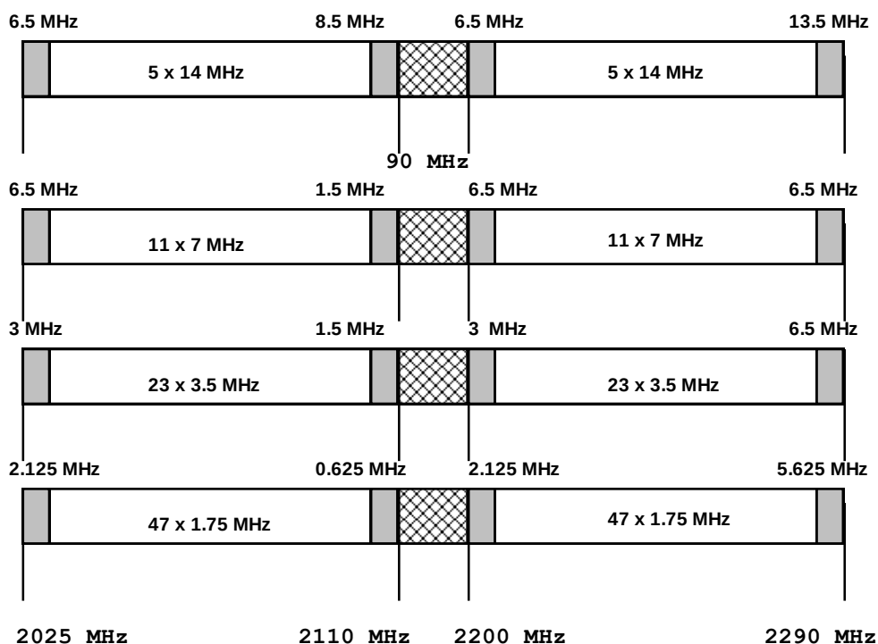
Figura 4. Brezi i frekuencave 2025 – 2110 MHz / 2200 – 2290 MHz
