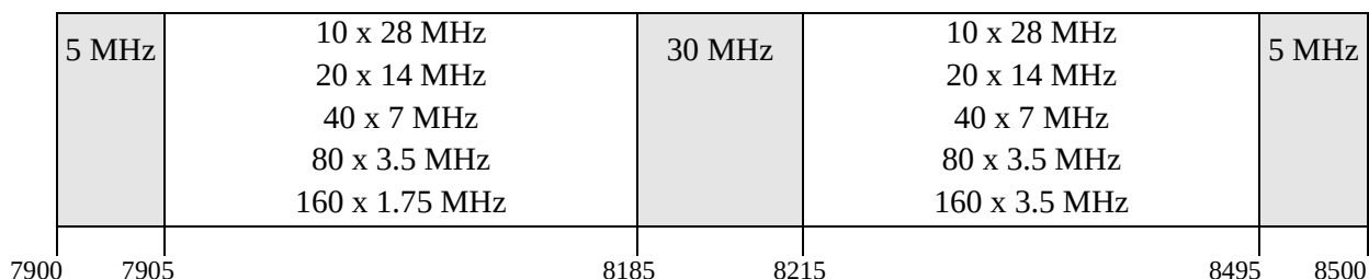
Figura 13. Brezi i frekuencave 7900 – 8500 MHz
