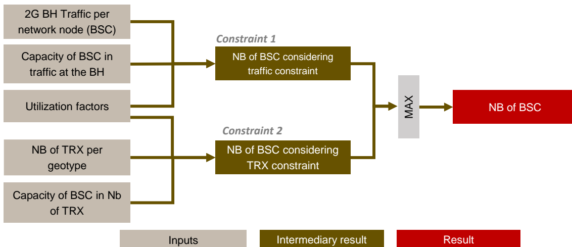
Figure 16 - BSC dimensioning
