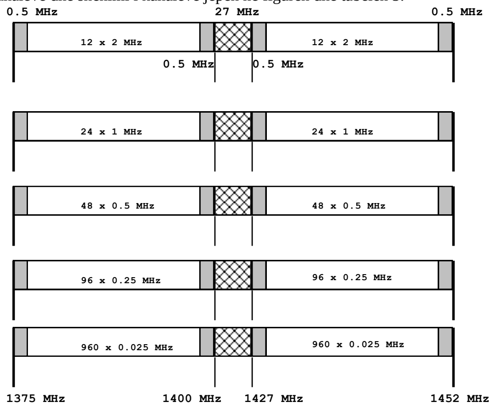
Figura 3. Brezi i Frekuencave 1375 – 1400 MHz / 1427 – 1452 MHz
