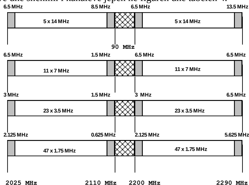
Figura 4. Brezi i frekuencave 2025 – 2110 MHz / 2200 – 2290 MHz
